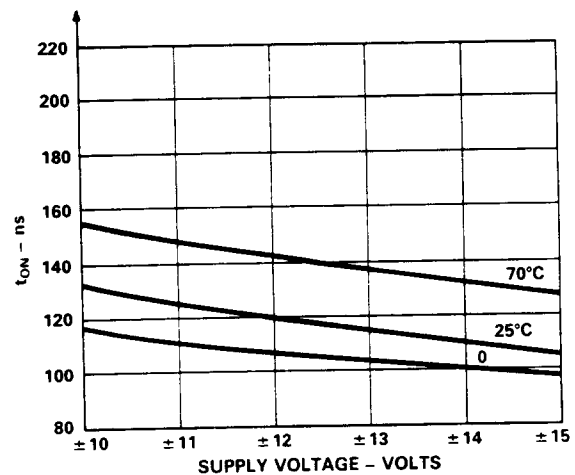
Figure 8. t_{ON} vs. Supply Voltage, (Dual Supply)
