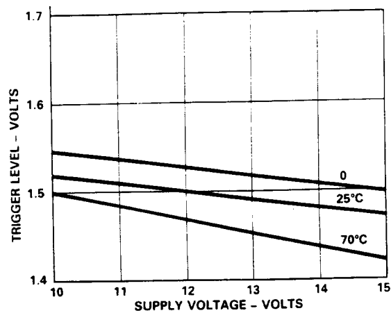
Figure 7. Trigger Levels vs. Power Supply Voltage, Dual or Single Supply Voltage
