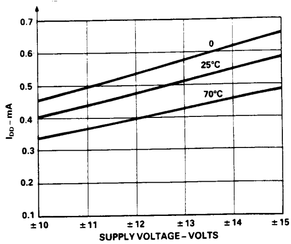
Figure 15. I_{DD} vs. Supply Voltage, (Dual Supply)
