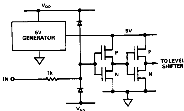
Figure 6. Digital Input Schematic
