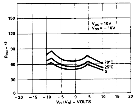
Figure 4. R_{ON} as a Function of V_D ( V_S ): Dual \pm 10V Supplies
