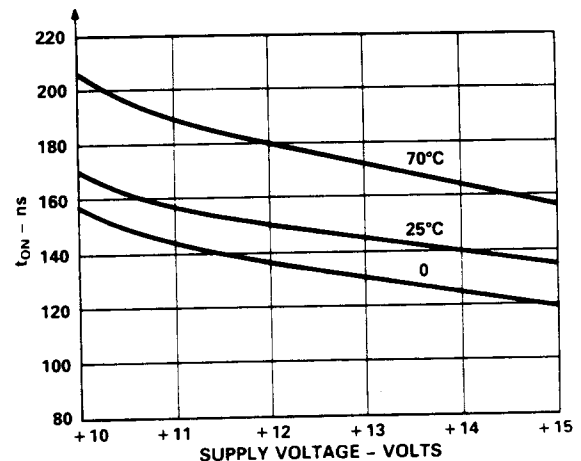
Figure 9. t_{ON} vs. Supply Voltage, (Single Supply)
