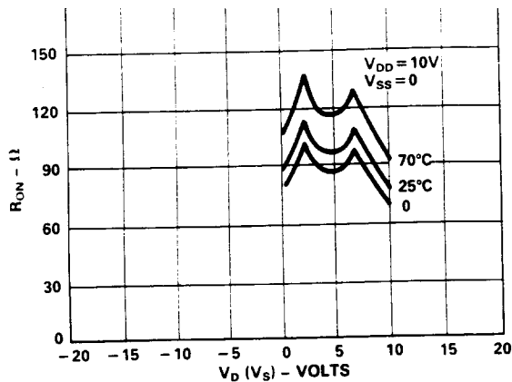
Figure 5. R_{ON} as a Function of V_D ( V_S ): Single +10V Supply
