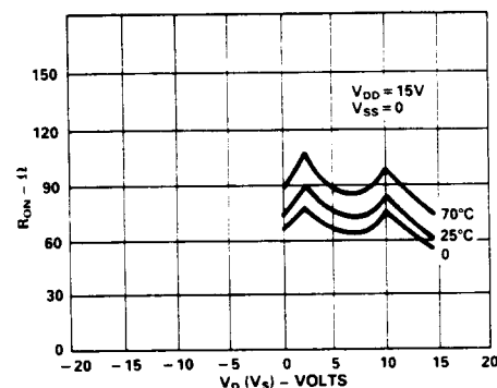
Figure 3. R_{ON} AS A FUNCTION OF V_D ( V_S ): Single +15V Supply
