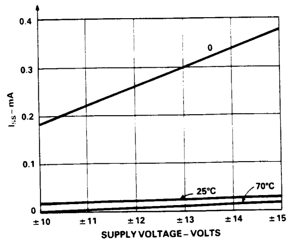
Figure 16. I_{SS} vs. Supply Voltage, (Dual Supply)
