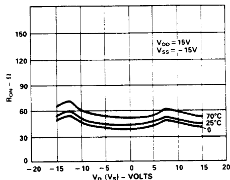
Figure 2. R_{ON} as a Function of V_D ( V_S ): Dual \pm 15 Supplies
