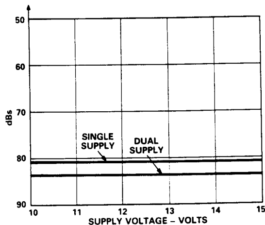
Figure 12. Off Isolation and Channel-to-Channel Crosstalk vs. Supply Voltage
