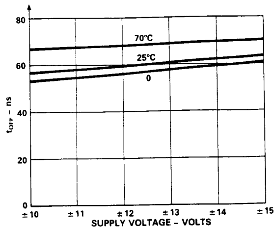
Figure 10. t_{OFF} vs. Supply Voltage, (Dual Supply)
