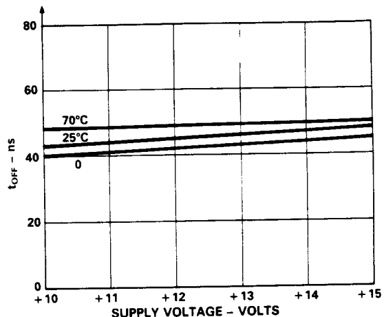
Figure 11. t_{OFF} vs. Supply Voltage, (Single Supply)
