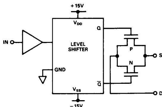
Figure 1. Output Switch Schematic
